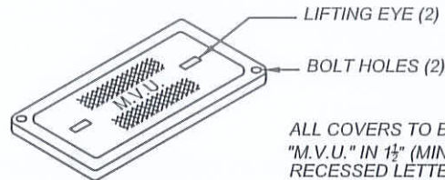
TYPICAL COVER (CONCRETE OR PLASTIC)
