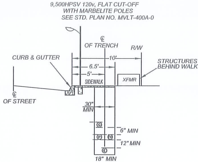
TRENCH DETAIL RESIDENTIAL & COLLECTOR STREETS
