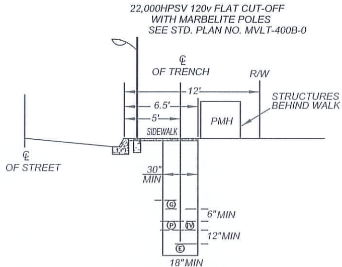
TRENCH DETAIL ARTERIAL STREET
